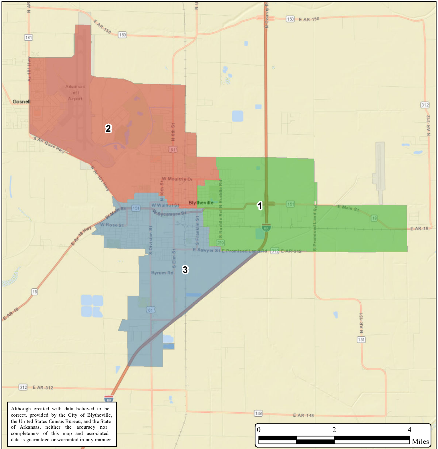
Population Statistics
